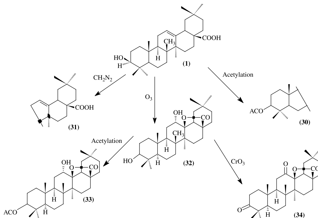
Scheme 6.
