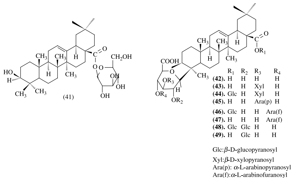
Scheme 8.
