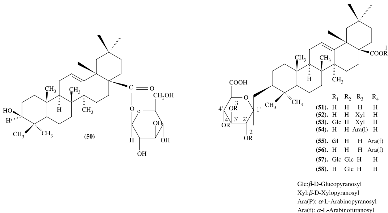
Scheme 9.
