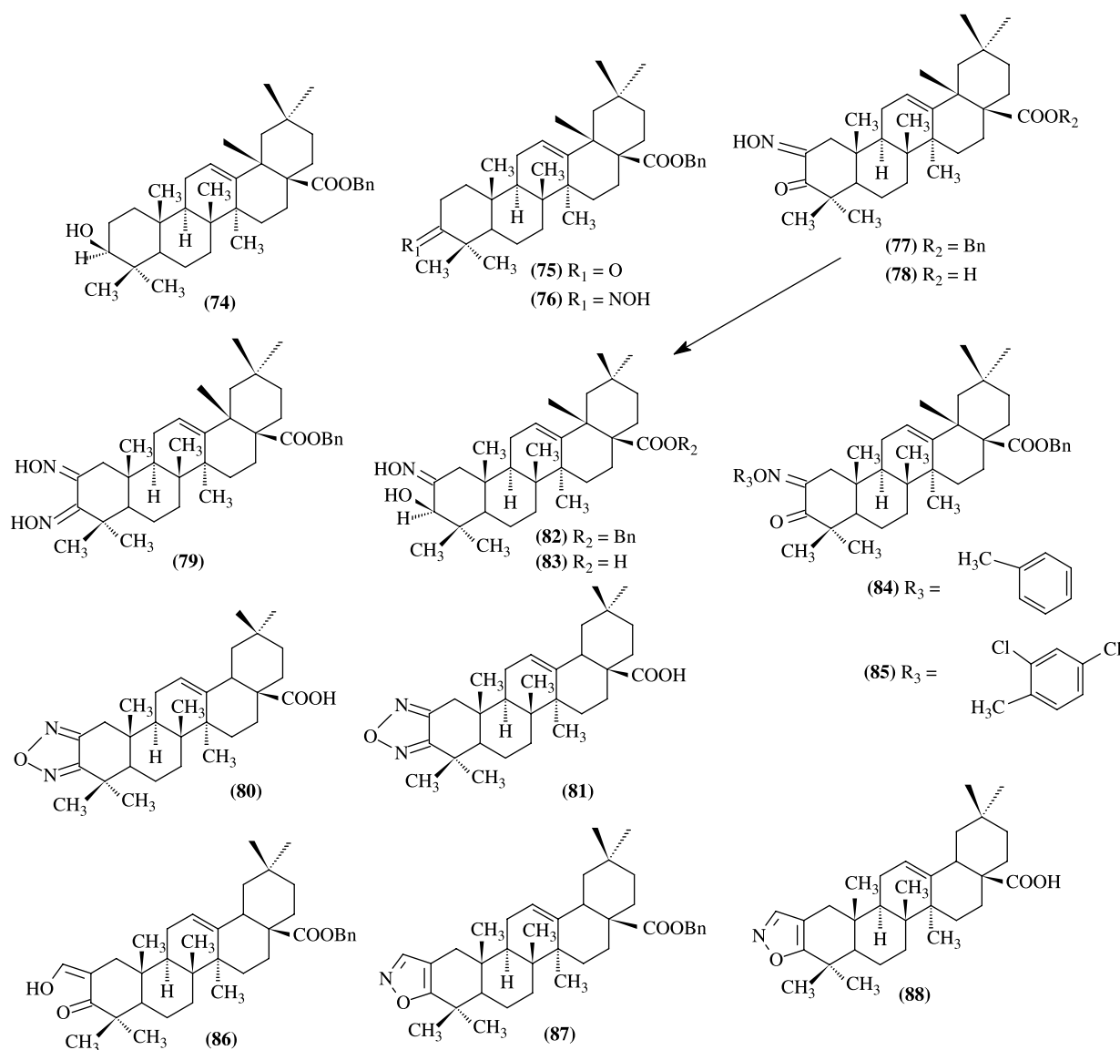
Scheme 11.
